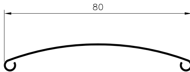
MV80C BLADE
